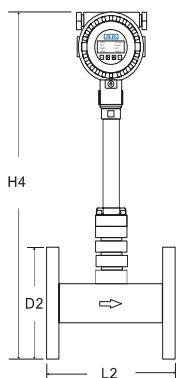
Flange Type Under Pressure Replace Sensor
