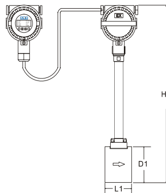
Separate Type
