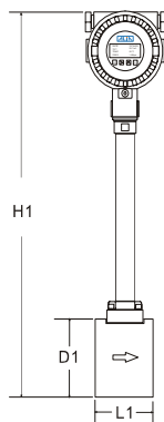
Wafer Type
